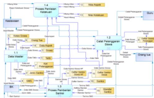
Gambar 7. Data Flow Diagram level 0
