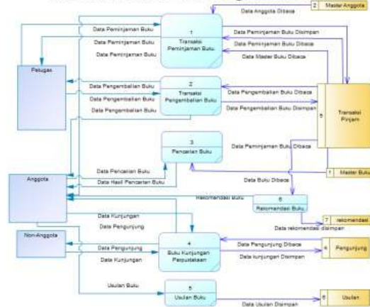
Gambar 7 Data Flow Diagram Level 1
