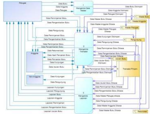
Gambar 6 Data Flow Diagram Level 0
