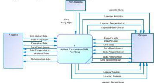
Gambar 8 Context Diagram
