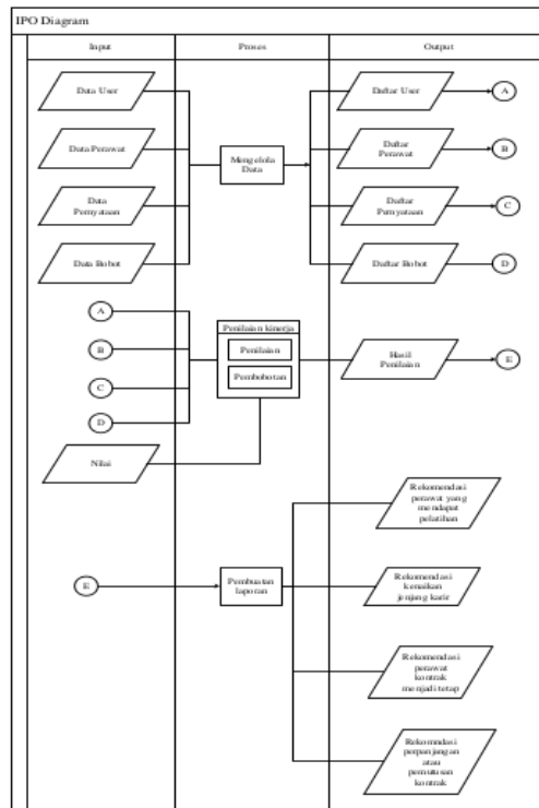
Gambar 2 Diagram Input Output
