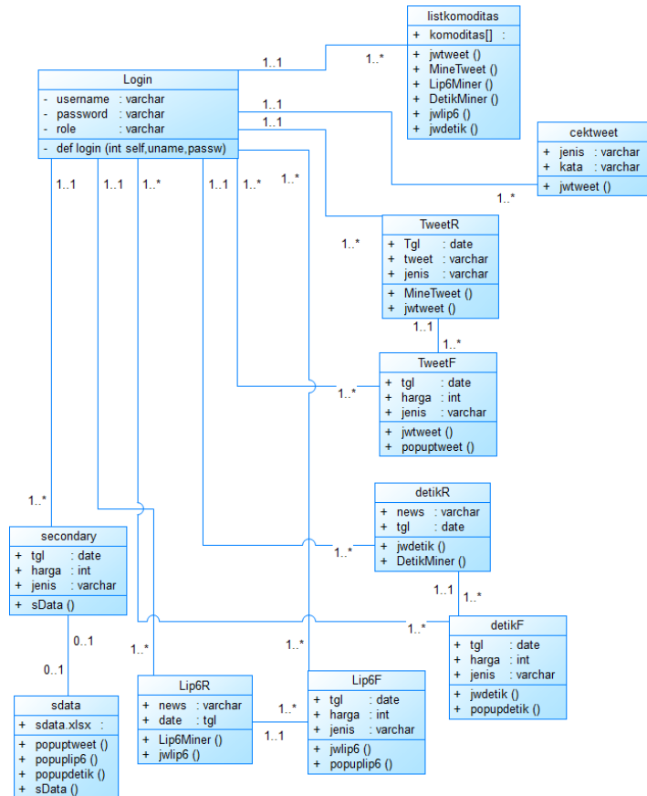
Gambar 5 Class Diagram
