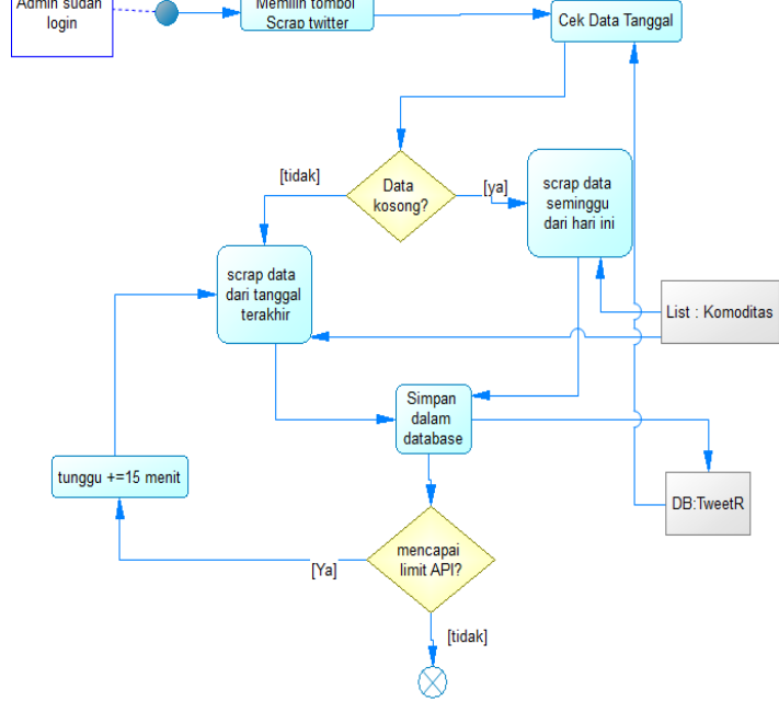
Gambar 3 Activity Diagram Scrapping Twitter
