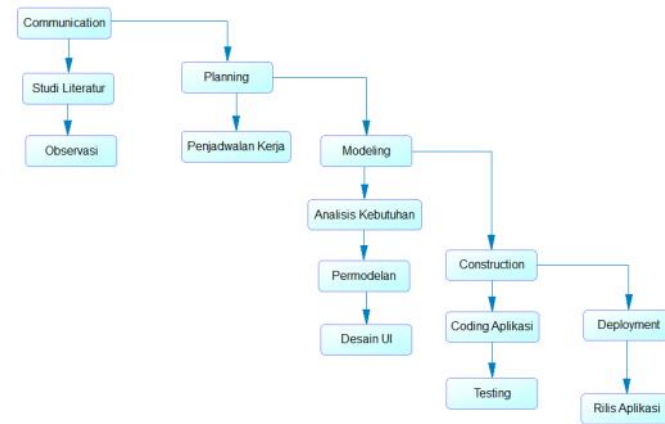
Gambar 1 SDLC Waterfall
