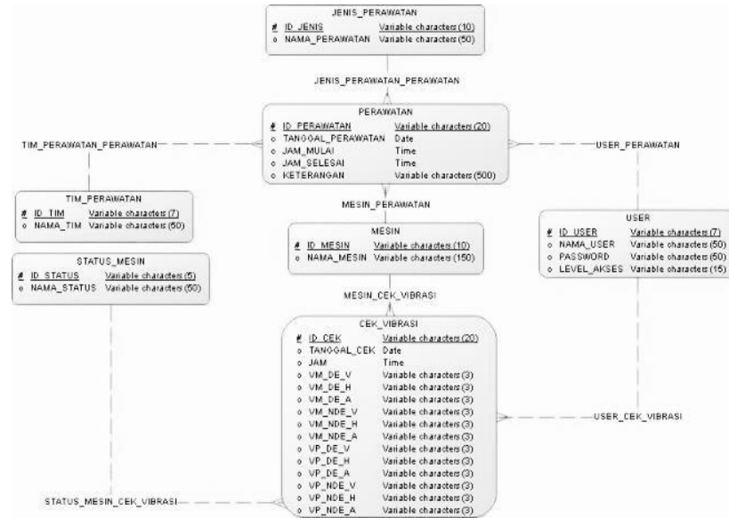
Gambar 4. Conceptual Data Model
