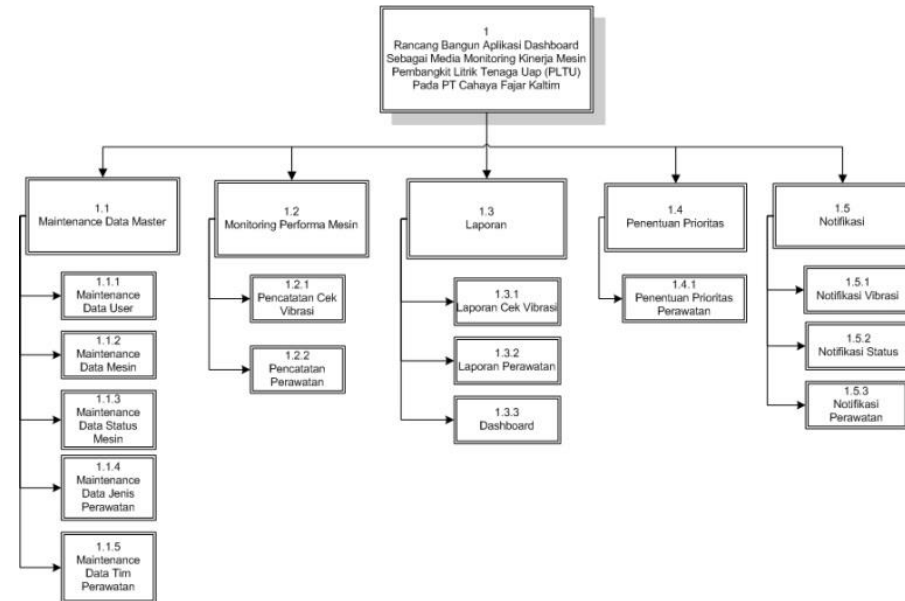
Gambar 3. Hierarchy Input Process Output (HIPO)
