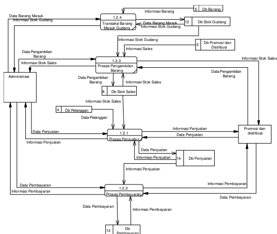
Gambar 10. Data flow diagram level 1 Transaksi
