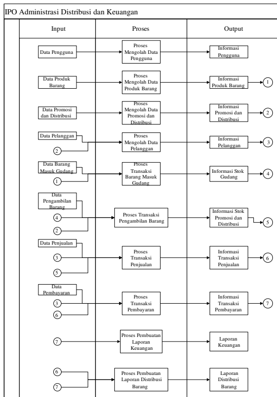
Gambar 2. Diagram IPO
