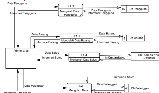
Gambar 9. Data flow diagram level 1 mengolah data
