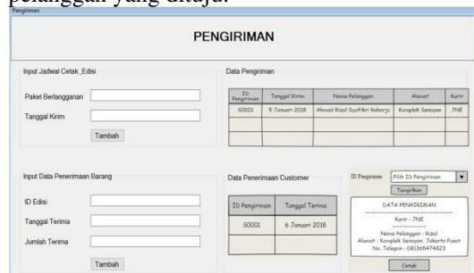
Gambar 8. Halaman Pengiriman
