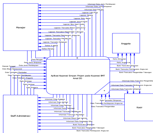
Gambar 6. Context Diagram
