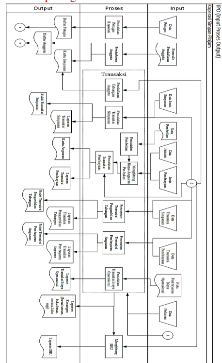
Gambar 5. IPO Diagram
