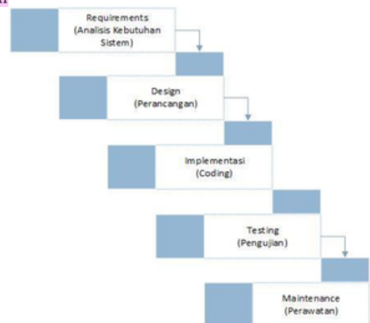
Gambar 1 SDLC Waterfall
