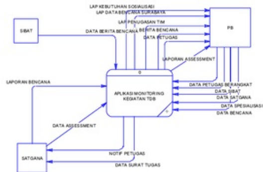
Gambar 6 Context Diagram
