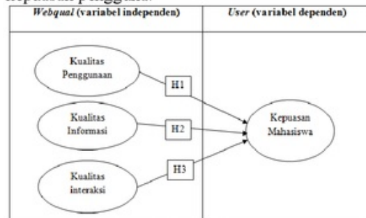
Gambar 4. Model Hipotesis
