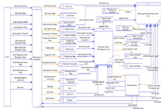
Gambar 3 DFD Level 0
