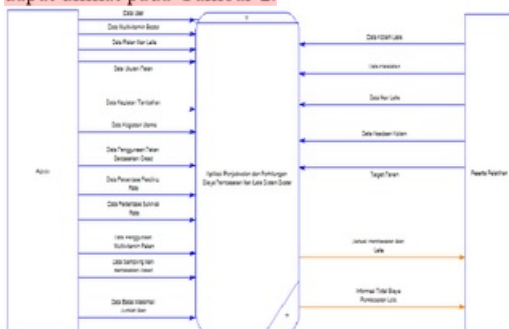
Gambar 2 Context Diagram
