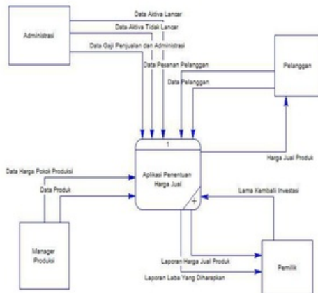
Gambar 3. Context Diagram
