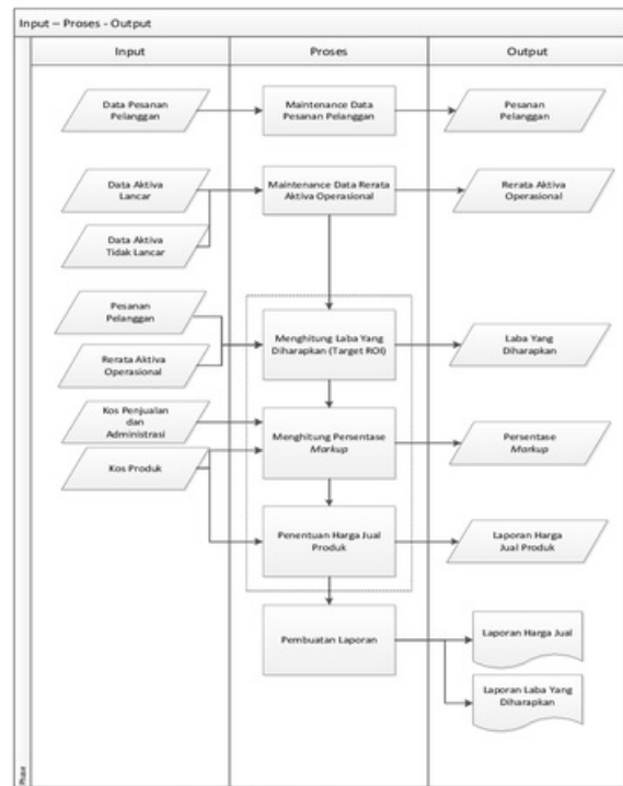
Gambar 2. IPO Diagram
