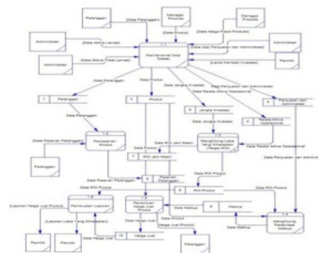
Gambar 4. DFD Level 0
