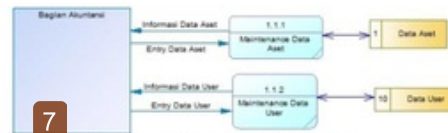
Gambar 5. DFD Level 1 Maintenance
