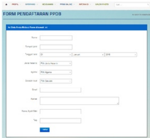
Gambar 9. Form PPDB
