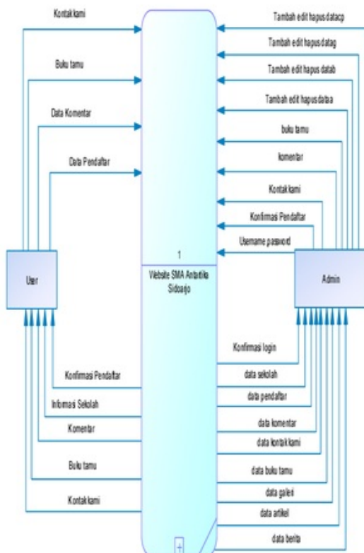
Gambar 2. Context Diagram
