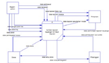
Gambar 7 Context Diagram
