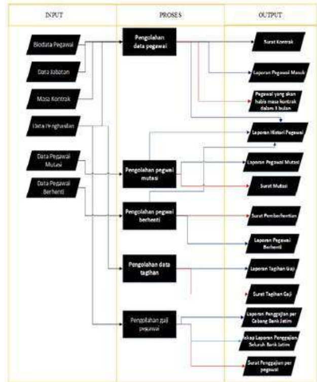
Gambar 2. Diagram Input-Process-Output (IPO)
