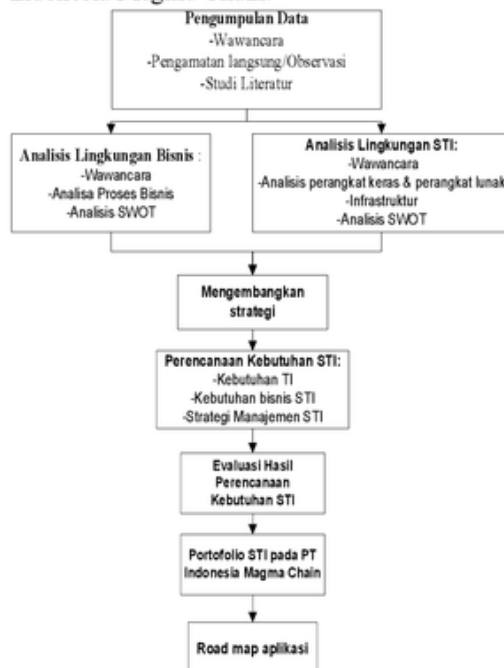
Gambar 1 Metode Penelitian
