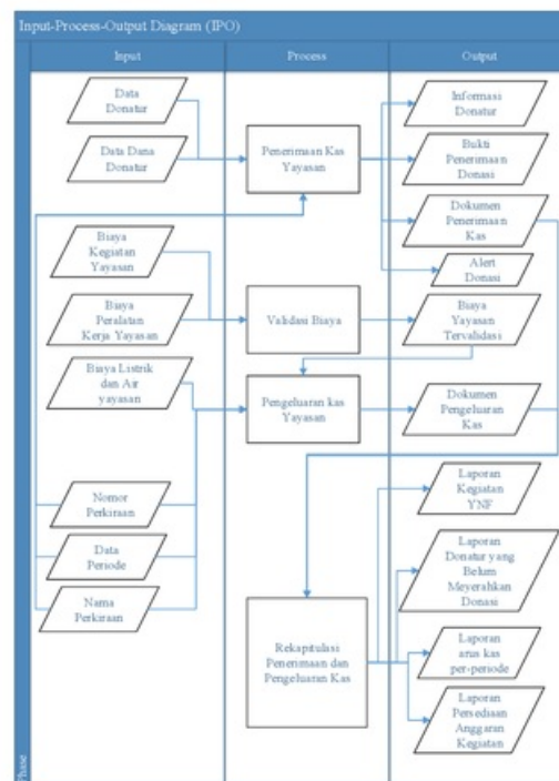
Gambar 2. Input-Process-Output (IPO) Diagram
