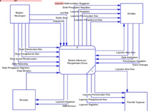
Gambar 3. Context Diagram
