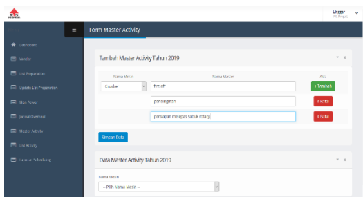
Gambar 7. Form tambah master activity.
