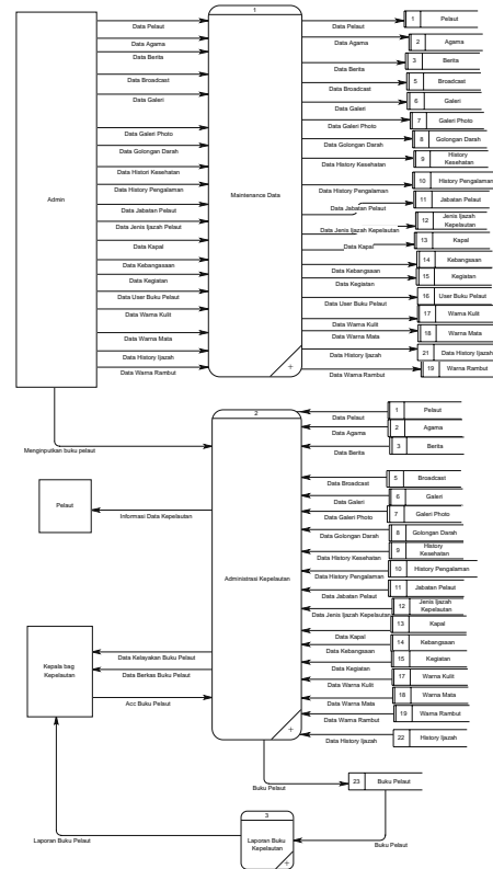
Gambar 8 DFD Level 1 Subproses
