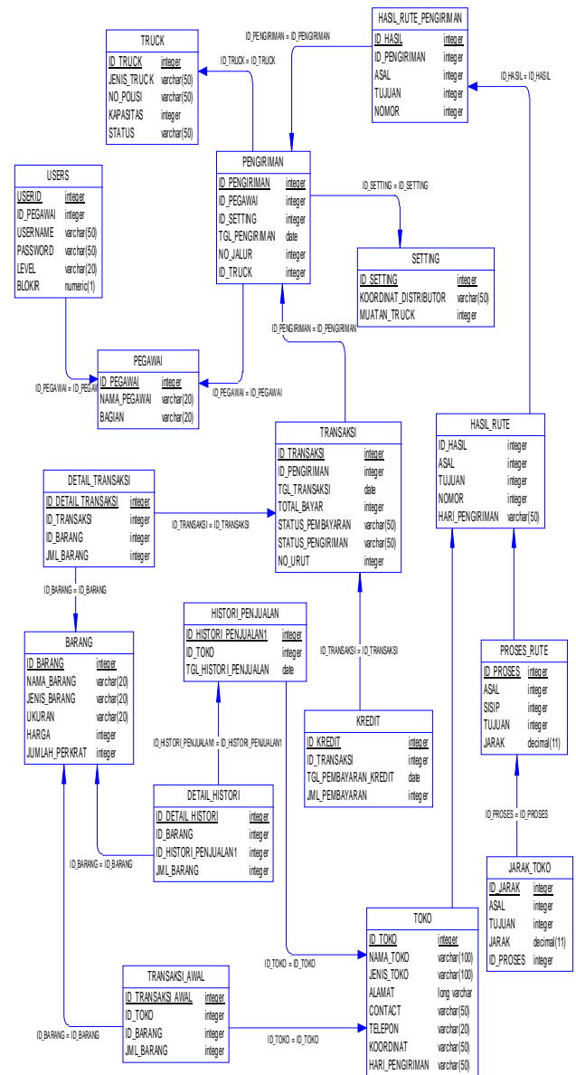
Gambar 6 Physical Data Model (PDM)
