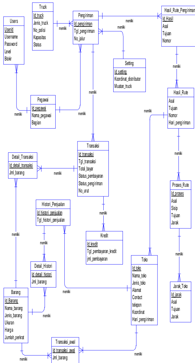
Gambar 5 Conceptual Data Model
