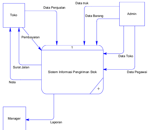
Gambar 2 Context Diagram Sistem Informasi Distribusi Stock
