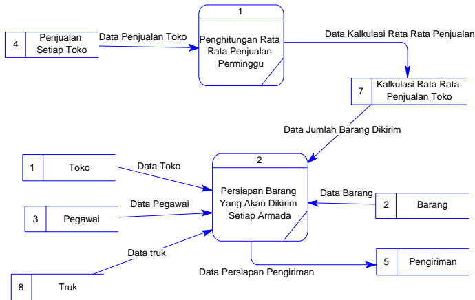
Gambar 4 DFD Level 1 Sub Proses Sistem Persiapan Pengiriman
