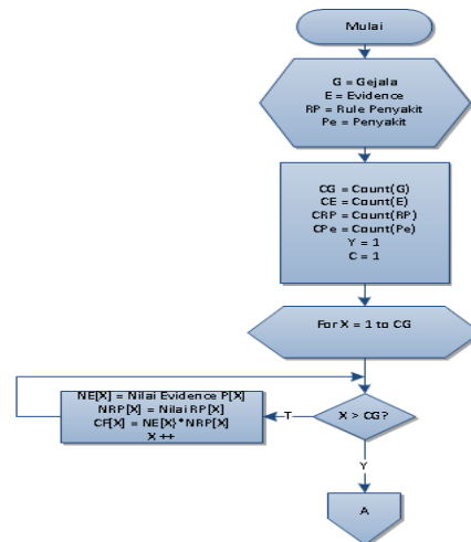
Gambar 1. Flowchart perhitungan nilai CF gejala
