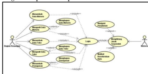
Gambar 1. Use Case Diagram (Adjie, 2021)
