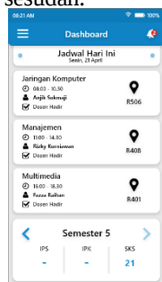
Gambar 15 Dashboard
