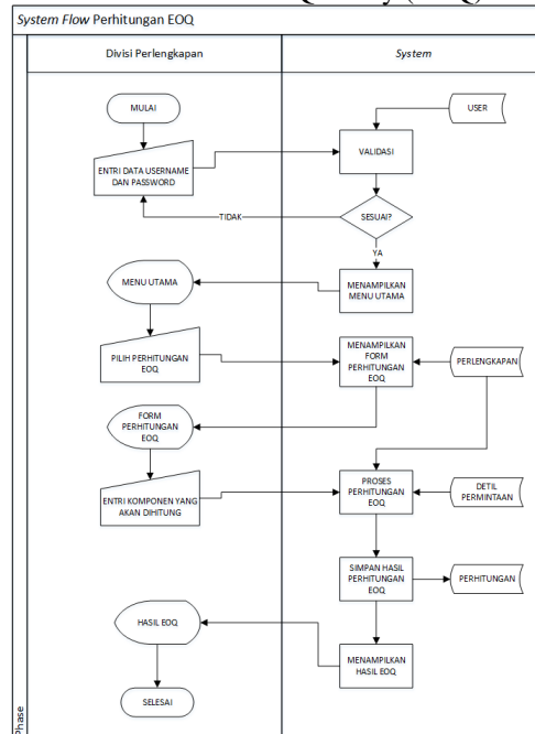
Gambar 4 System Flow Perhitungan EOQ
