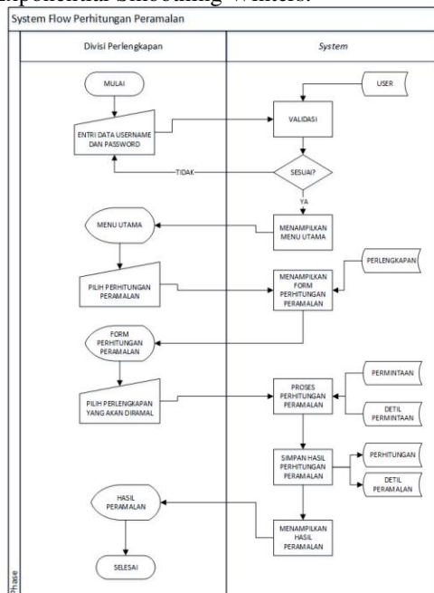
Gambar 3 System Flow Perhitungan Peramalan
