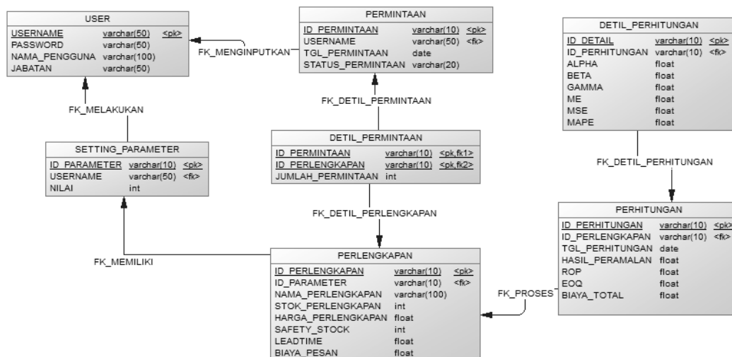
Gambar 7 Physical Data Model (PDM)
