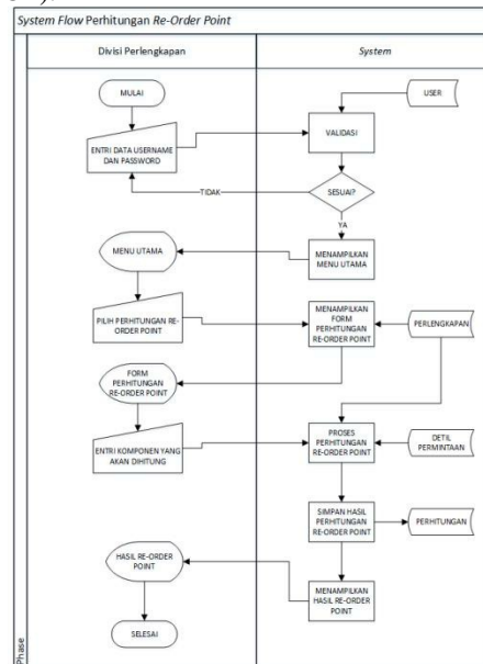
Gambar 4 System Flow Perhitungan ROP
