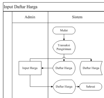
Gambar 6. System Flow Daftar Harga
