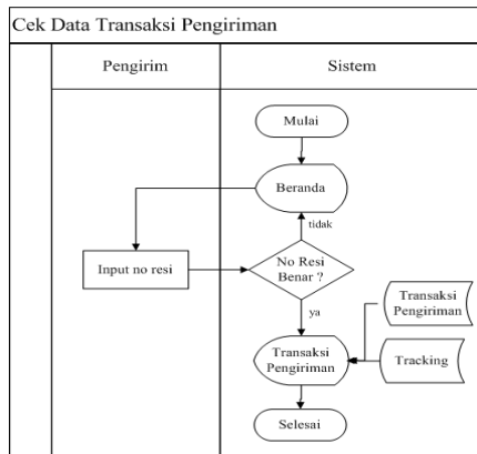
Gambar 7. System Flow Cek Pengiriman
