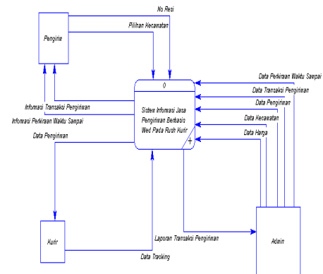
Gambar 9. Context Diagram Jasa Pengiriman
