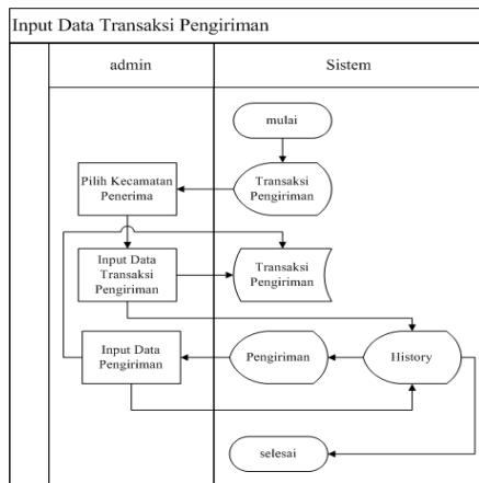
Gambar 3. System Flow Input Transaksi Pengiriman
