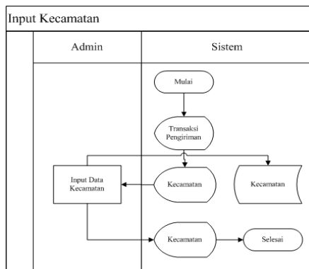
Gambar 4. System Flow Proses Kecamatan
