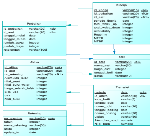
Gambar 2 Physical Data Model
