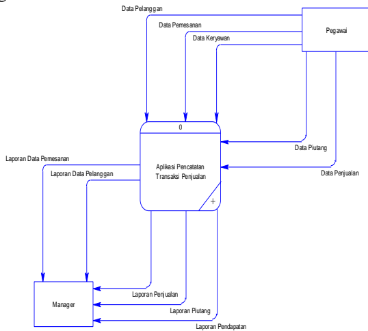
Gambar 2 Context Diagram
