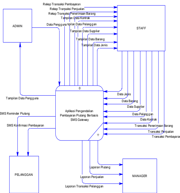
Gambar 3 Context Diagram
