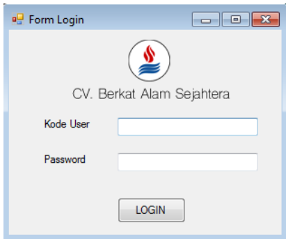
Gambar 6 Form Login
